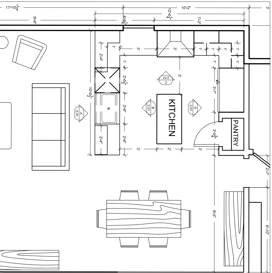
DRAKE KITCHEN FLOOR PLAN SCALE 1/4"=1'
