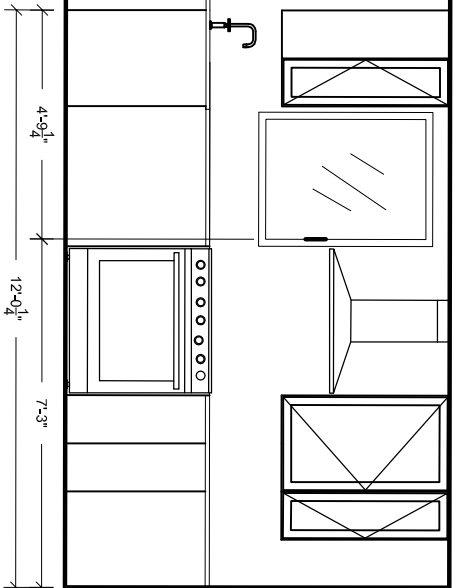
ELEVATION C / 2.01 SCALE 1/2"=1'
